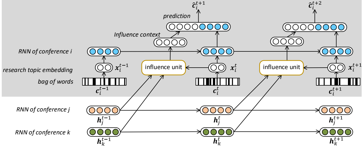
Figure 2: The framework of Correlated Neural Influence Model.
