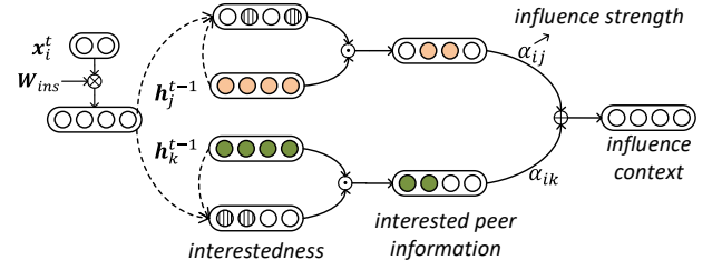
Figure 3: The scientific influence unit. The dotted lines are aimed to capture i 's interestedness on the research outcomes of its peers \mathbf{h}_j^{t-1} and \mathbf{h}_k^{t-1} , which is denoted by Eq. 7. The solid lines illustrate that after selecting the peer research outcomes with the interestedness, the interested peer information is combined under the influence strength \alpha_{ij} and \alpha_{ik} , forming the influence context, which is denoted by Eq. 8 and 9.
